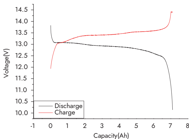
12.8V 20Ah Charge-Discharge Curve 0.2C, 25°C
